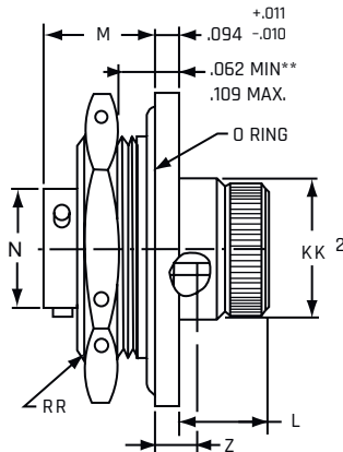
JT07RE-XX-XXX (MS27474E)
