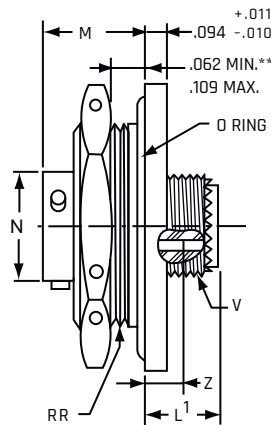
JT07RT-XX-XXX (MS27474T)
