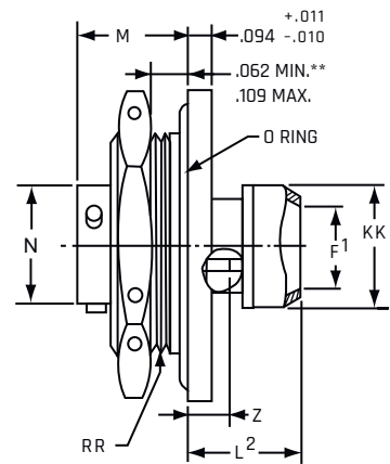
JT07RP-XX-XXX (MS27474P)
