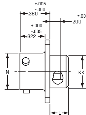
JT02RE-XX-XXX (MS27499)
