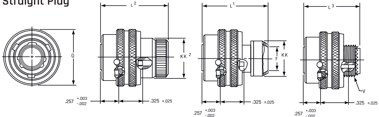
JT06RE-XX-XXX (MS27473E)
